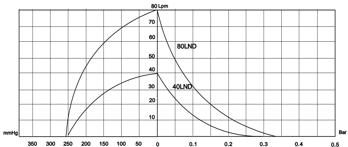
Oil-less Linear Diaphragm air Pump
